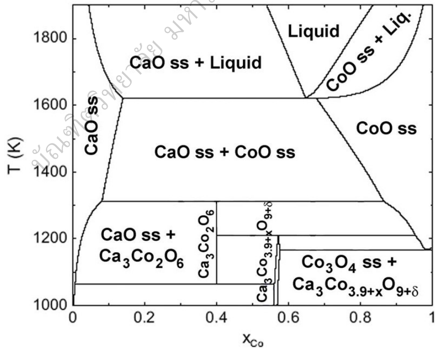
Figure 2.A The Ca–Co–O phase diagram under air atmosphere
