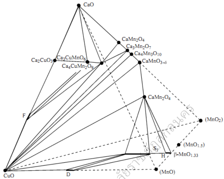
Figure 1.A The CaO–CuO–Cu 2 O–MnO–MnO 2 phase diagram
